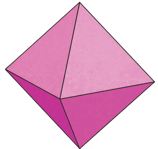
octahedron
