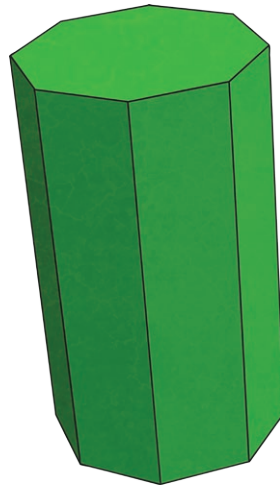
prism octagonol
