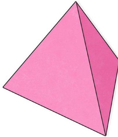
tetrahedron
